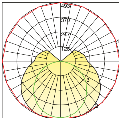
LN1-SL LINEA 1 SQUARE LENS
