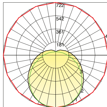
LN1-FRL LINEA 1 FLAT ROUNDED LENS
