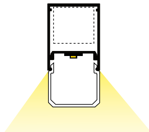
LN1-SL LINEA 1 SQUARE LENS
