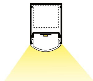
LN1-FRL LINEA 1 FLAT ROUNDED LENS
