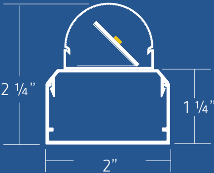
CV2A COVE 2 ASYMMETRIC
