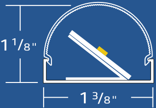
CV1A COVE 1 ASYMMETRIC
