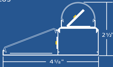
CV5+A COVE 5 PLUS ASYMMETRIC
