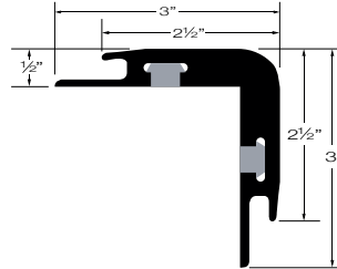
PL-LSL-C/C CARPET TO CARPET
