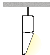
CSV (48 or 72") CABLE SUSPENDED VERTICAL
