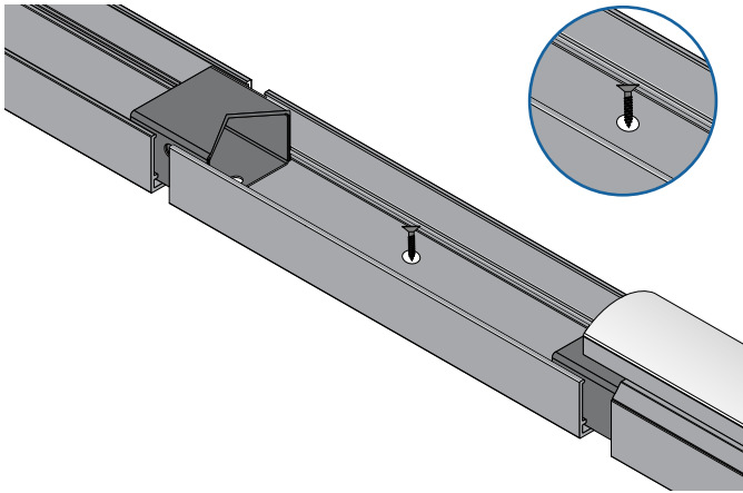
INSIDE SCREW MOUNT
