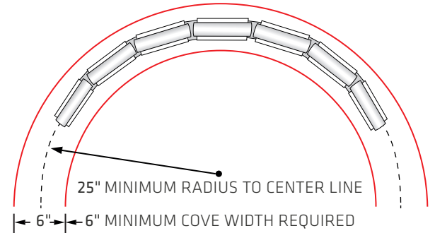
MINIMUM RADIUS AND COVE REQUIREMENTS
