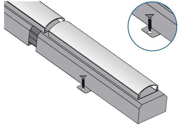
TAB MOUNT
