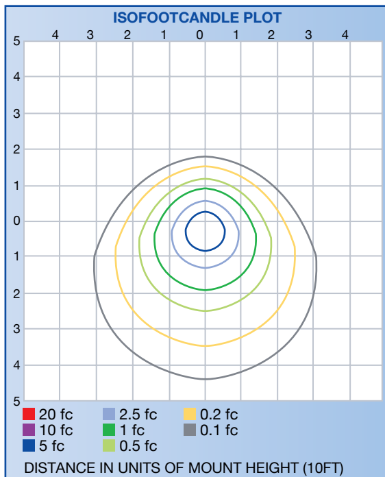
ISOILLUMINATION PLOT
