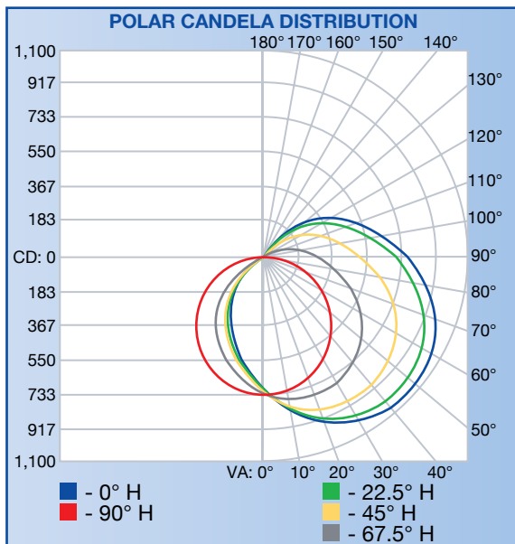
POLAR GRAPH
