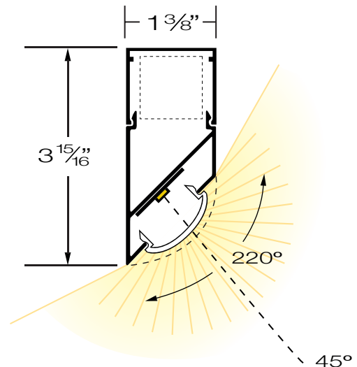
FIXTURE END VIEW
